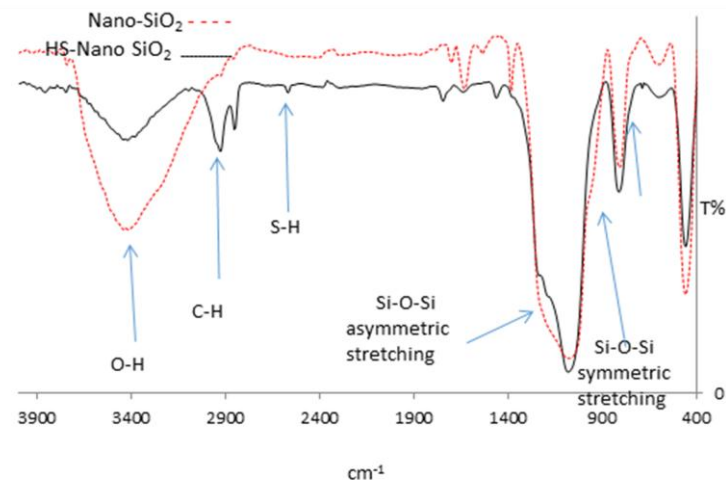
Figure 2- IR spectrum of the nanosilica (Si) and thiolated nanosilica (HS-Si) absorbent
